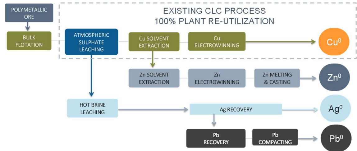
PMR Process Flow Chart
