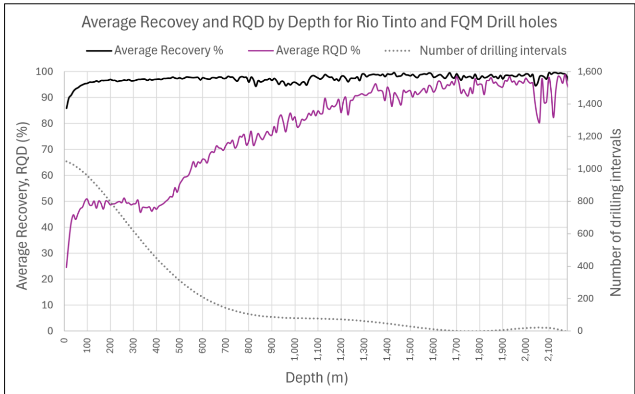
Figure 10-6 Core recovery and RQD by downhole depth for Rio Tinto and FQM drill holes (source: FQM)
