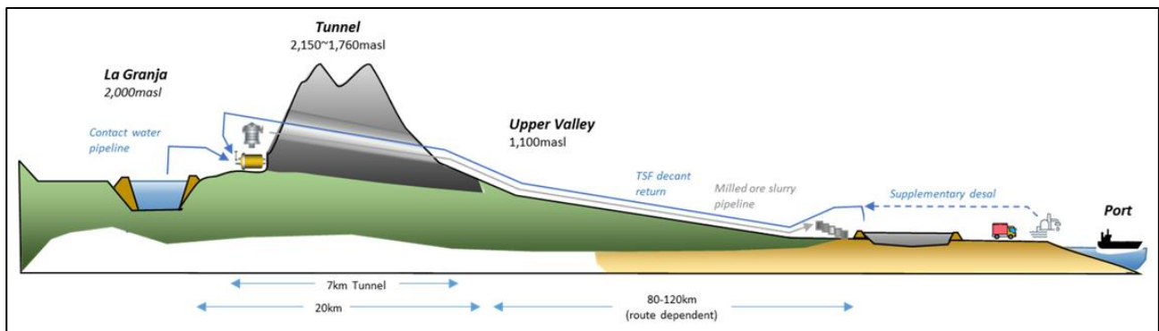
Figure 5-7 Conceptual infrastructure project layout (source: FQM)
