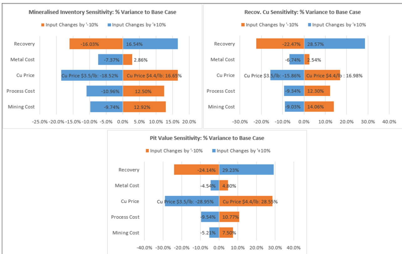
Figure 14-29 Key pit optimization sensitivities (source: FQM)
