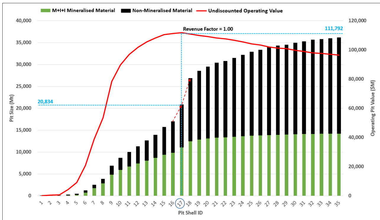
Figure 14-28 Pit optimization results (source: FQM)
