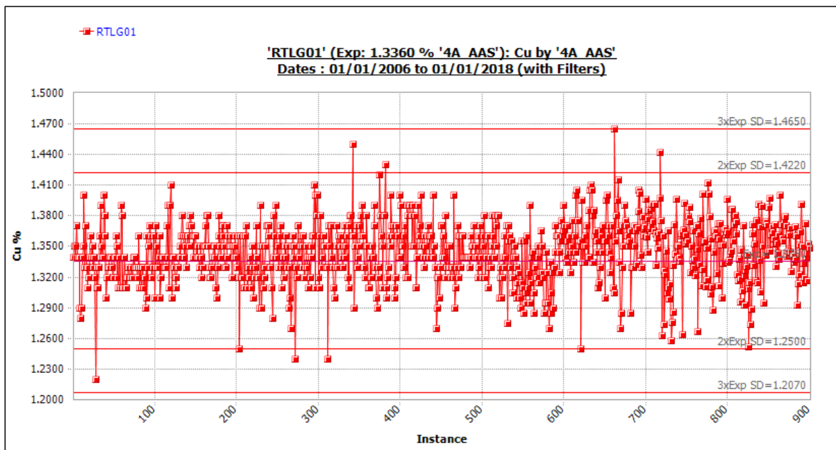
Figure 11-1 Control chart for RTLG01 used by Rio Tinto - copper values (source: Rio Tinto)
