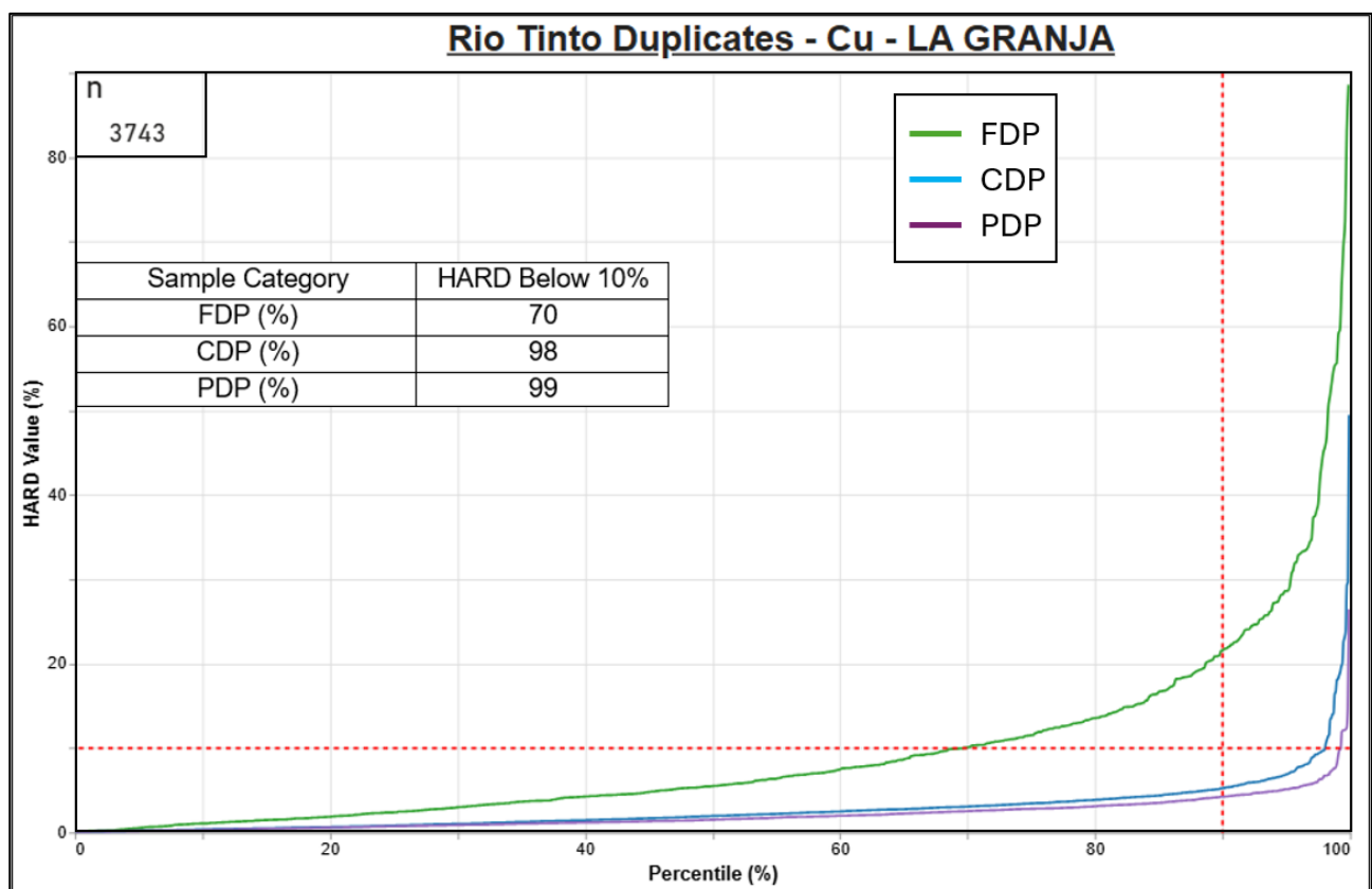
Figure 11-10 HARD plot – Rio Tinto copper duplicates (source: Rio Tinto)
