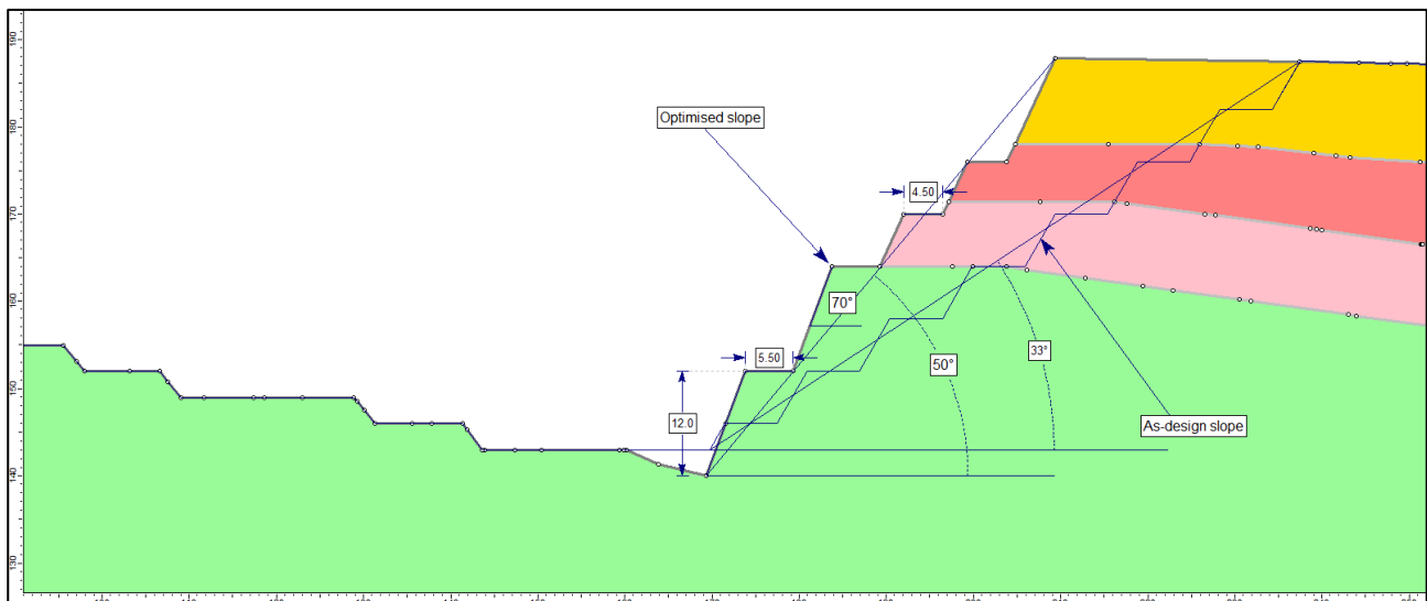
Figure 16-1 Shoemaker-Levy Recommended Pit Slopes
