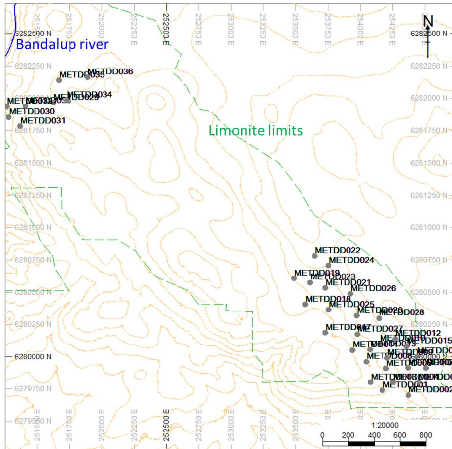
Figure 13-1 Plan view of the Diamond drilled holes used for beneficiation analysis at Shoemaker-Levy
