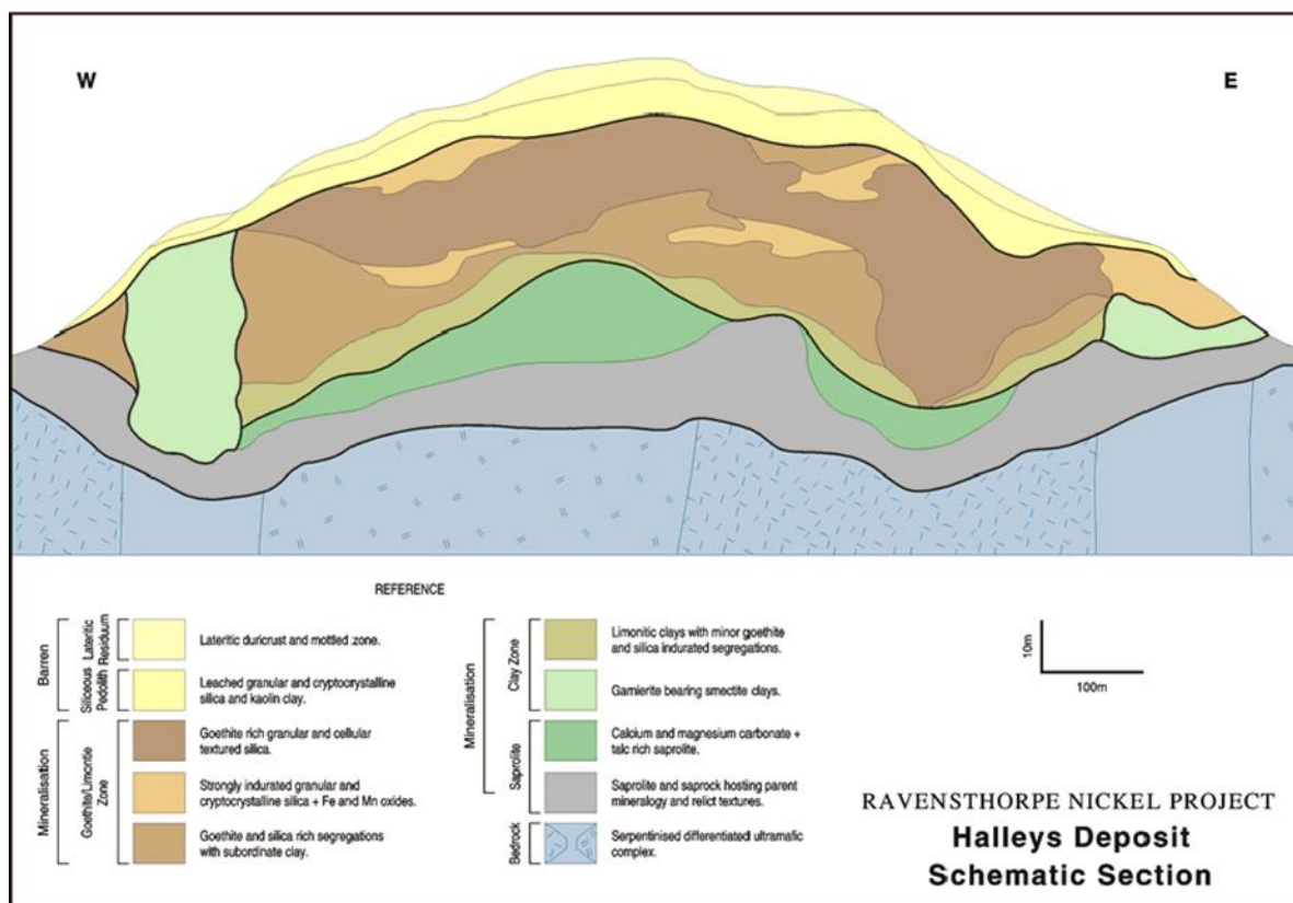
Figure 7-2 Schematic Section, Halleys Laterite Profile (BHP, 2003)
