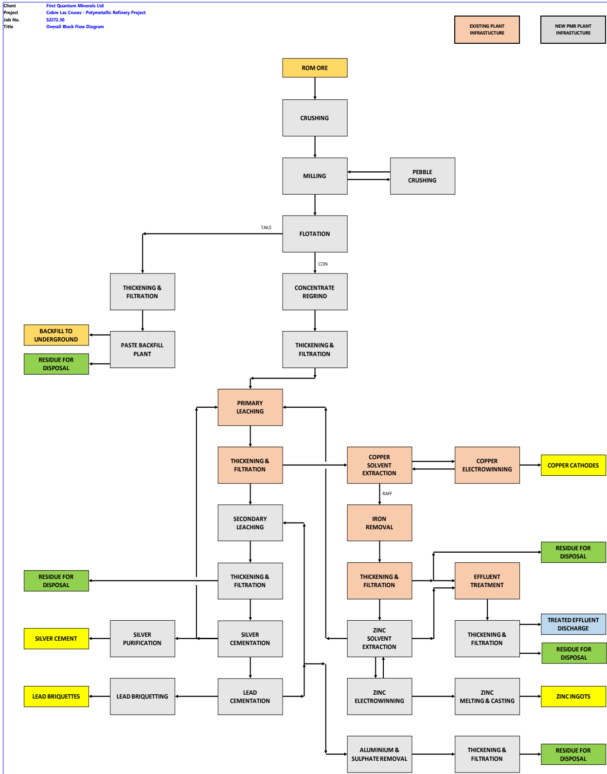
Figure 1-10 Overall Block Flow Diagram
