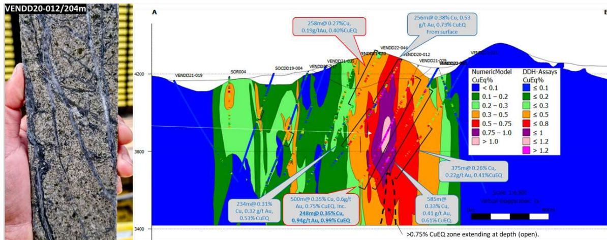
Figure 9 - Long Section view to NW of Vendaval Central with CuEq grades after phase IV, Lefthand image shows typical 'EMP' core.
